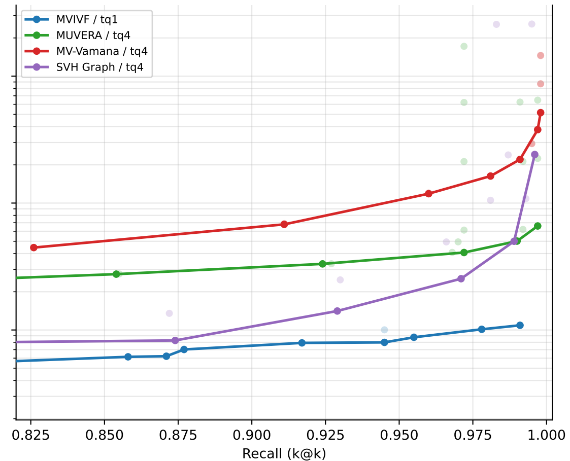
scifact: recall vs latency (1000 / QPS_seq ms) [multi_latency]
