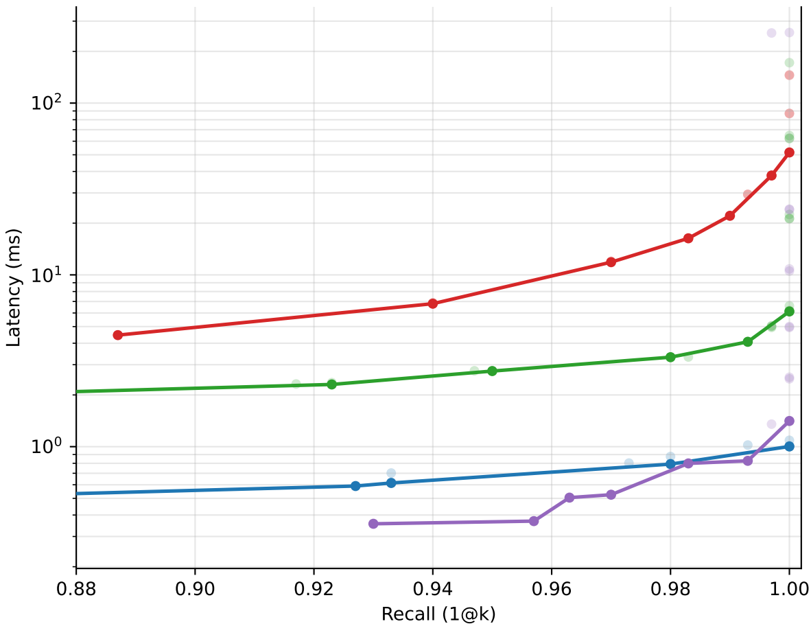
scifact: recall vs latency (1000 / QPS_seq ms) [multi_latency]
