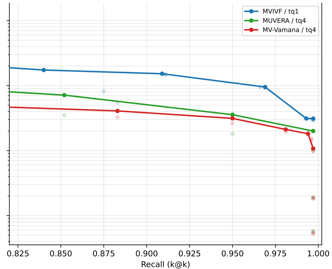
nfcopus: recall vs QPS [batch]
