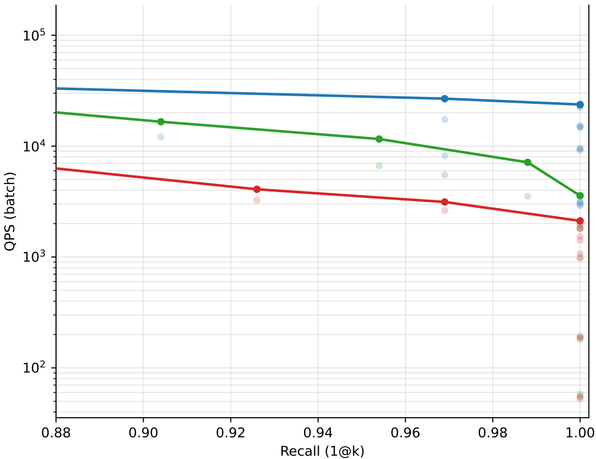
nfcopus: recall vs QPS [batch]
