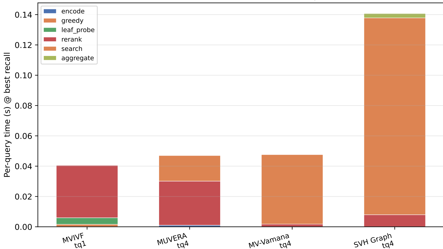
scifact: timer breakdown [latency]
