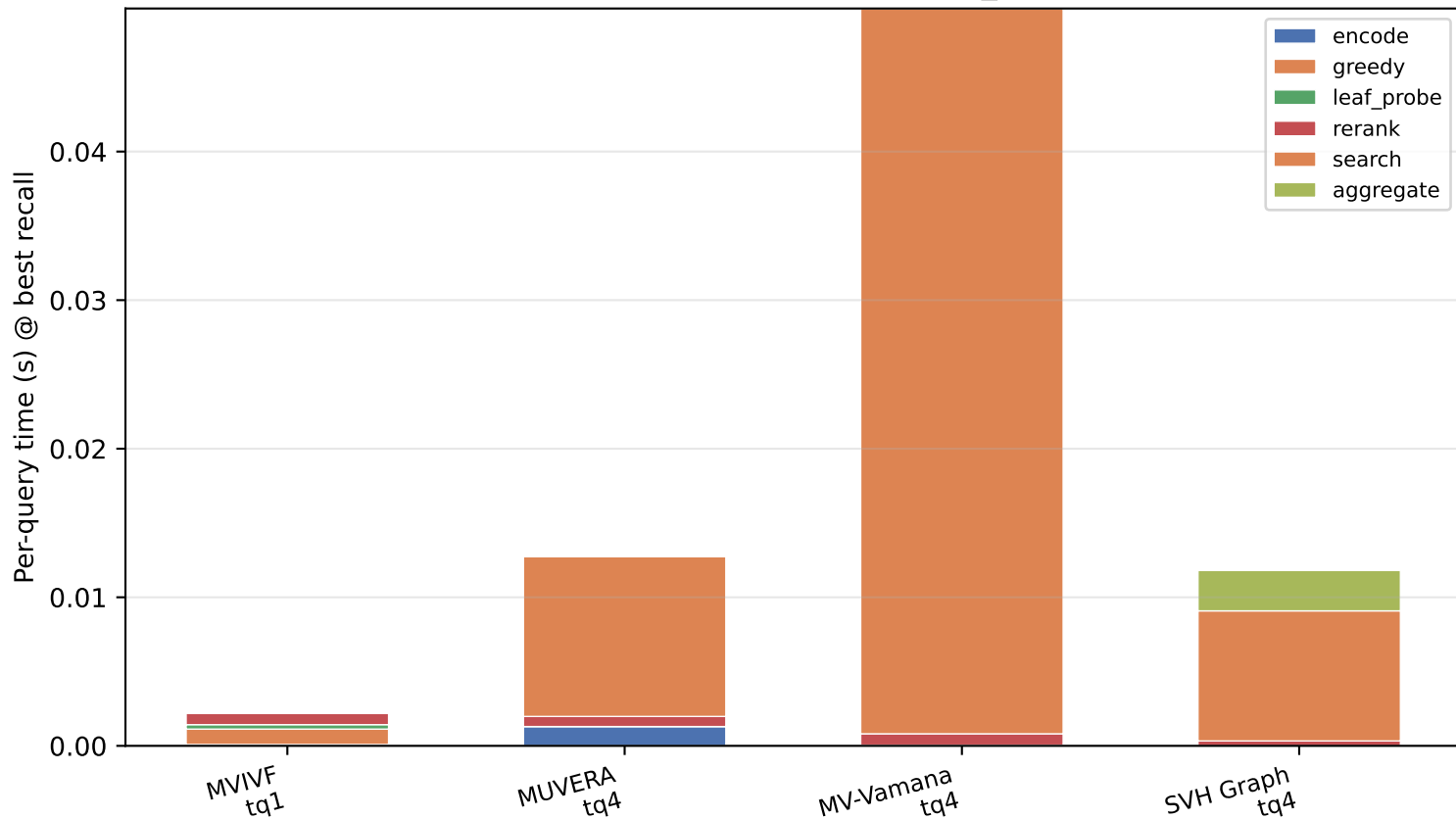
arguana: timer breakdown [multi_latency]
