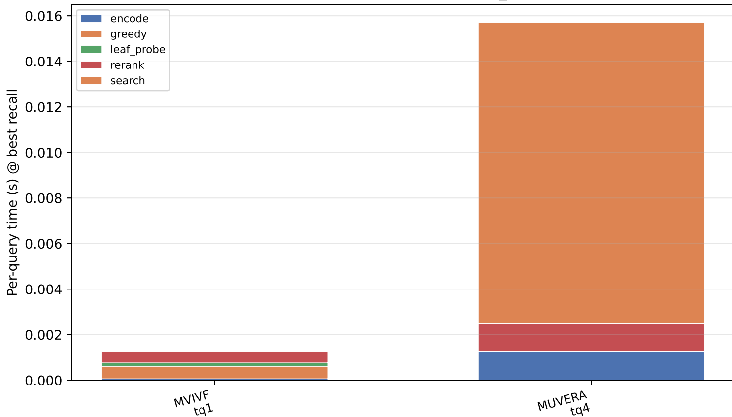
nfcopus: timer breakdown [multi_latency]
