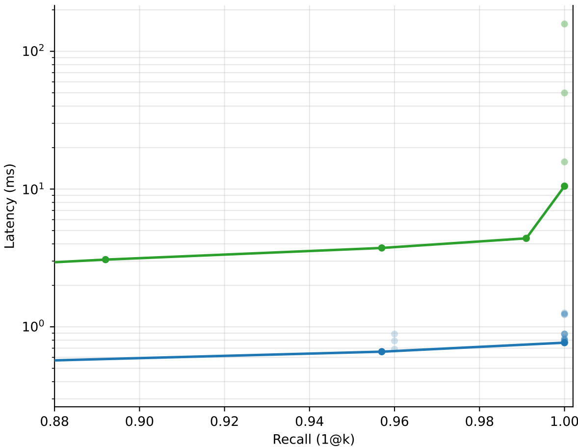
nfcopus: recall vs latency (1000 / QPS_seq ms) [multi_latency]
