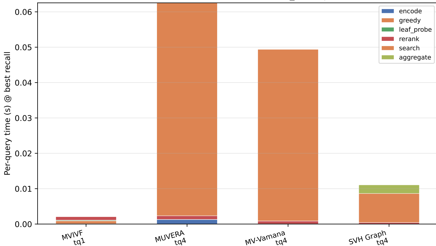
scifact: timer breakdown [multi_latency]
