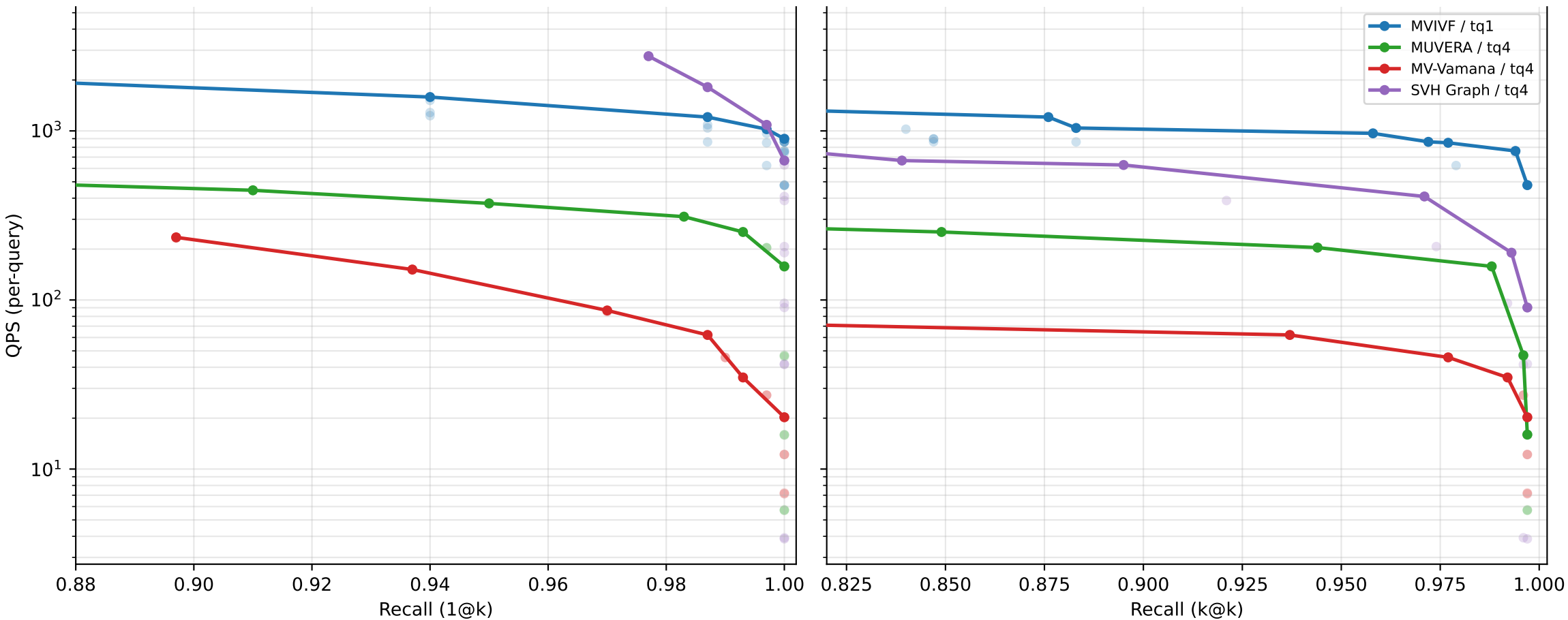
scifact: recall vs QPS [multi_latency]
