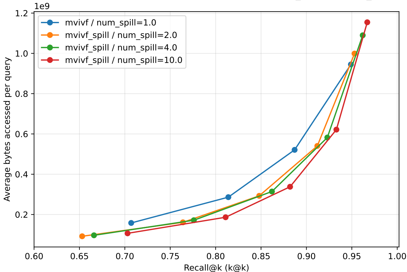
stage5: bytes accessed vs recall (grouped by index_name \times num_spill)
