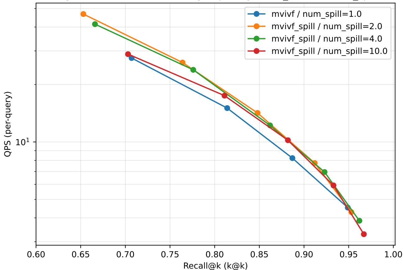
stage5: QPS vs recall Pareto (grouped by index_name × num_spill)
