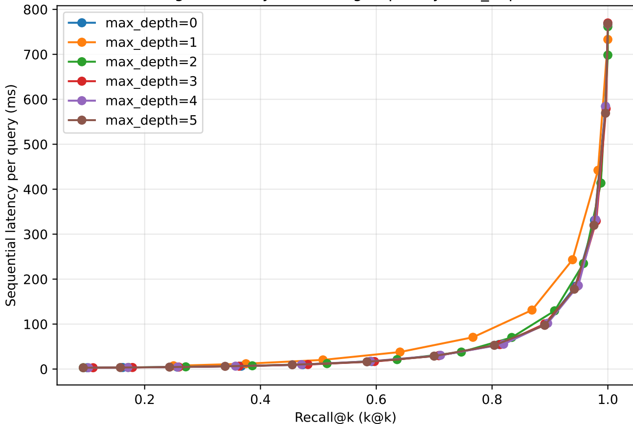
stage3: latency vs recall (grouped by max_depth)
