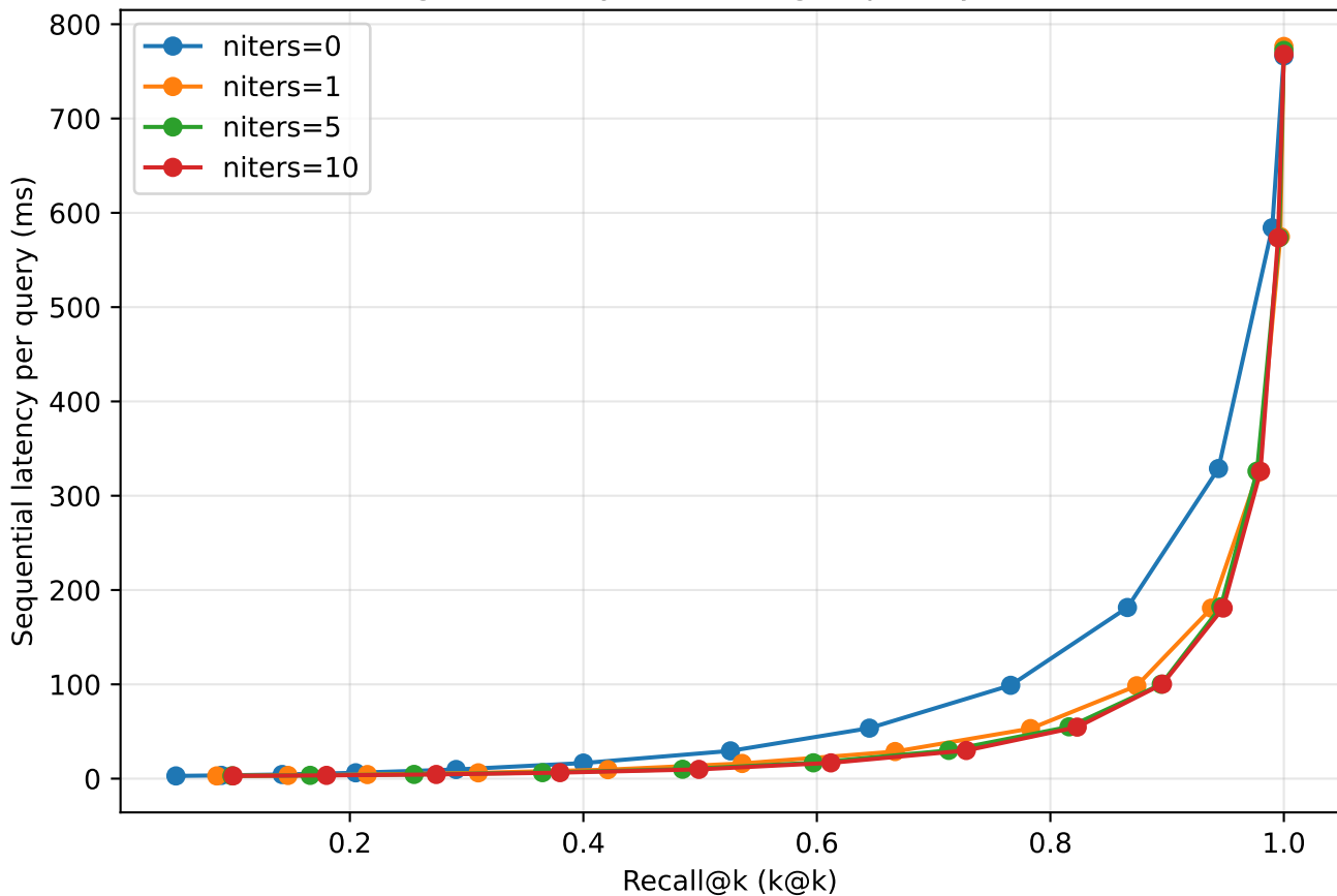
stage4: latency vs recall (grouped by niters)
