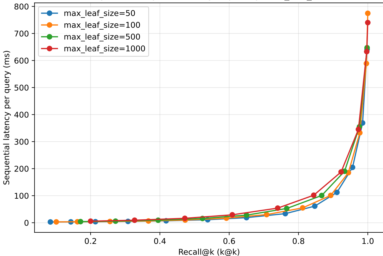
stage2: latency vs recall (grouped by max_leaf_size)
