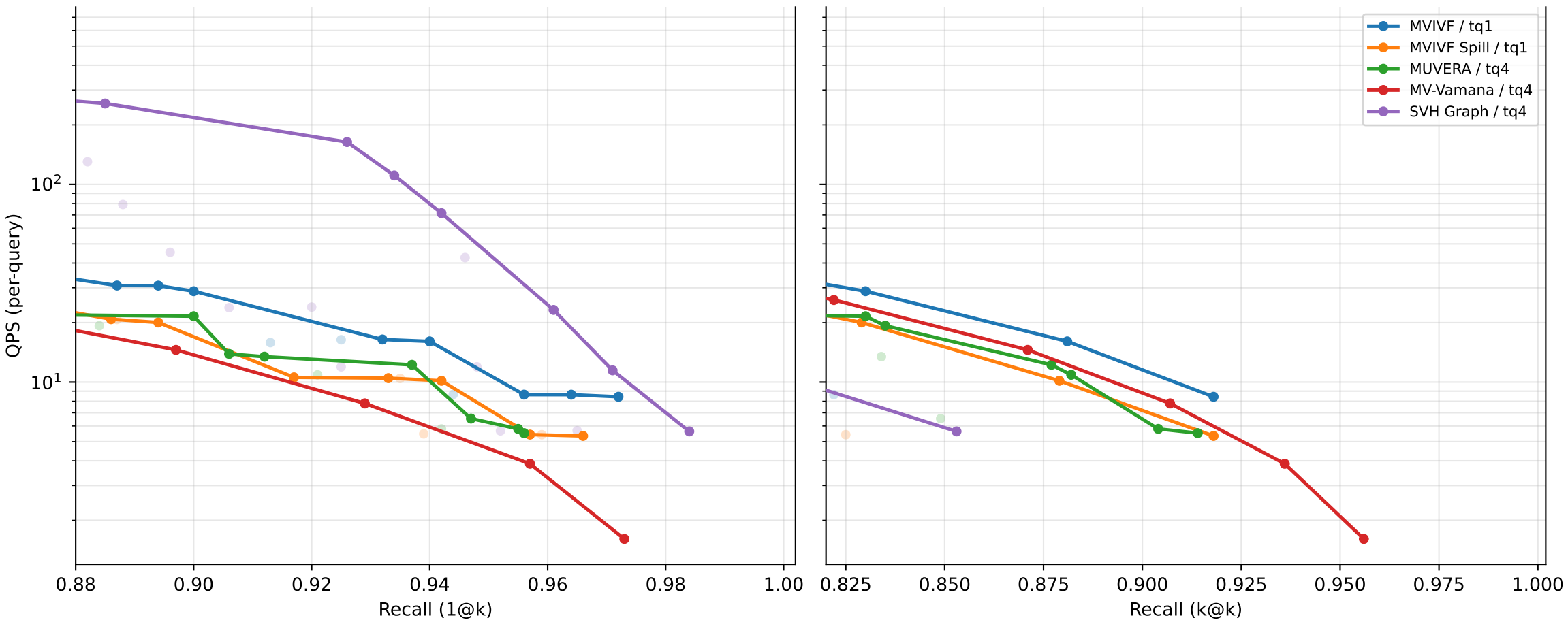
hotpotqa: recall vs QPS [latency]
