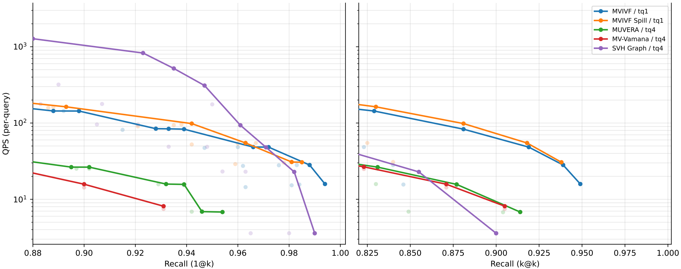
hotpotqa: recall vs QPS [multi_latency]
