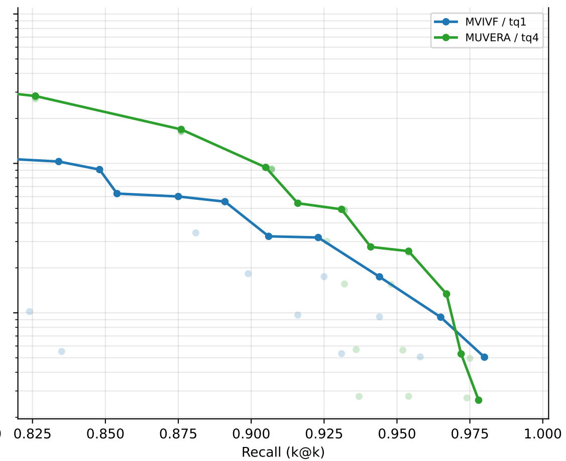
msmarco: recall vs QPS [batch]
