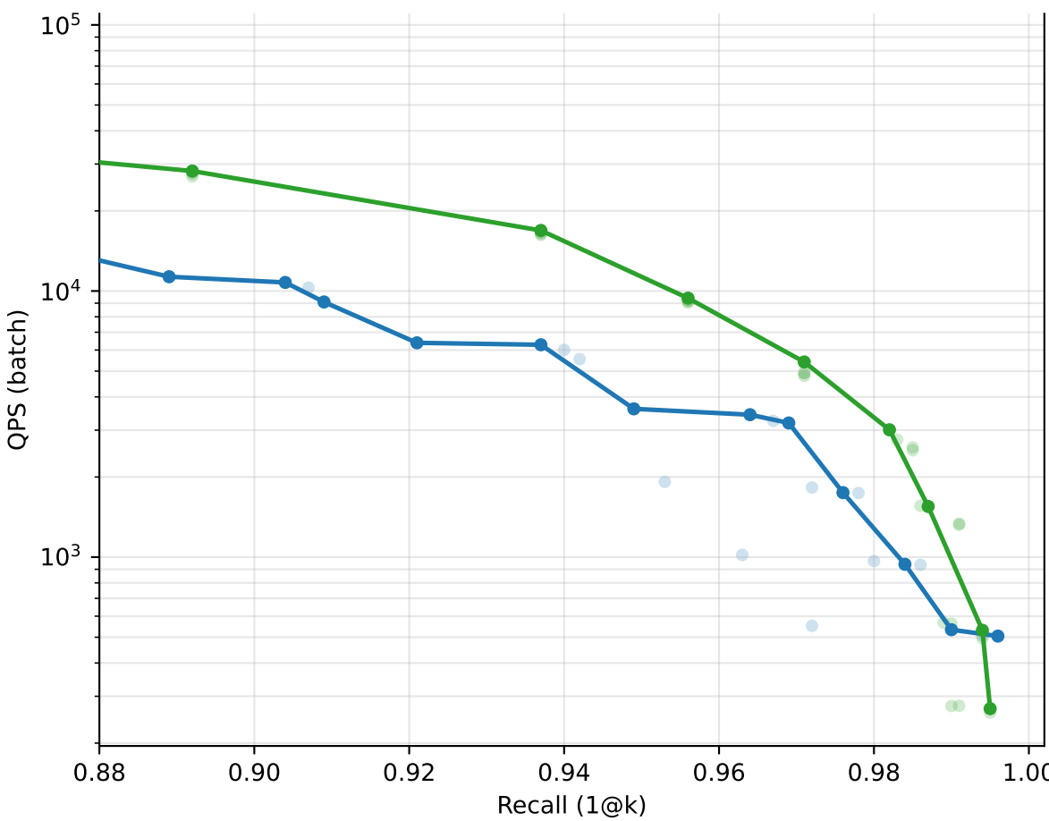
msmarco: recall vs QPS [batch]
