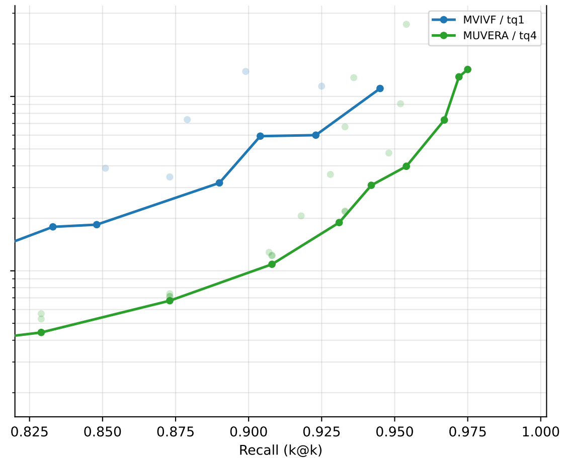
msmarco: recall vs latency (1000 / QPS_seq ms) [latency]
