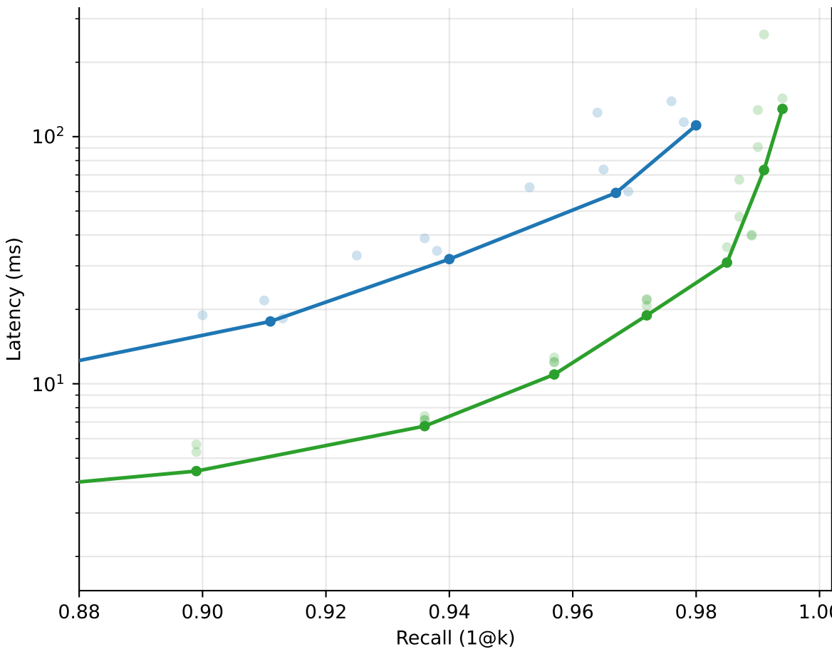
msmarco: recall vs latency (1000 / QPS_seq ms) [latency]
