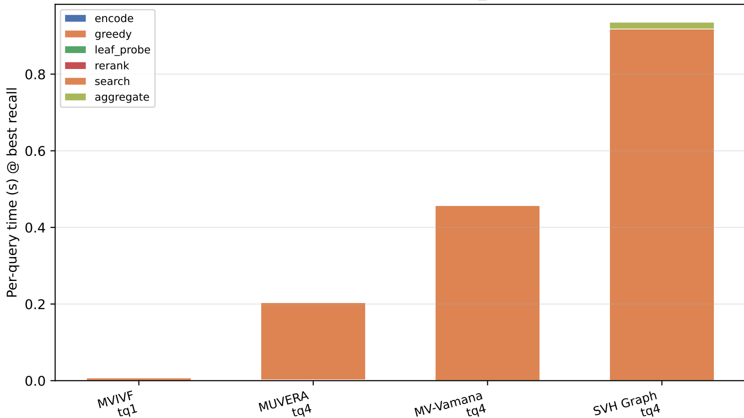
fiqa: timer breakdown [multi_latency]
