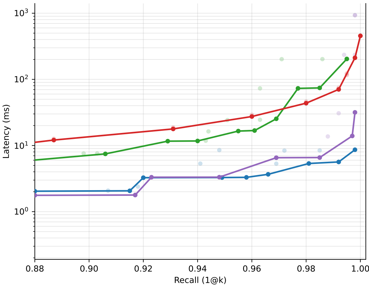
fiqa: recall vs latency (1000 / QPS_seq ms) [multi_latency]
