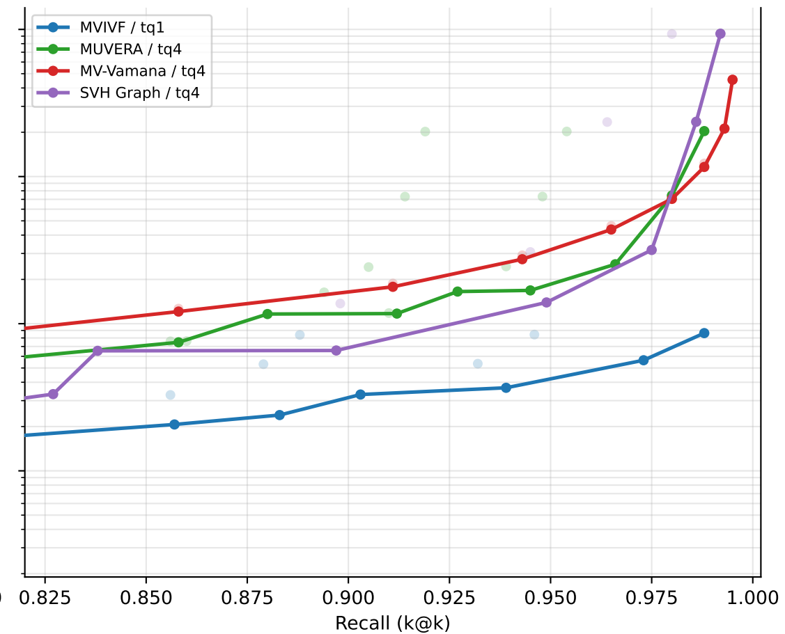
fiqa: recall vs latency (1000 / QPS_seq ms) [multi_latency]
