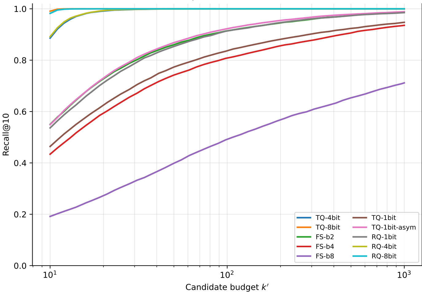
nfcopus: Recall@10 vs k'
