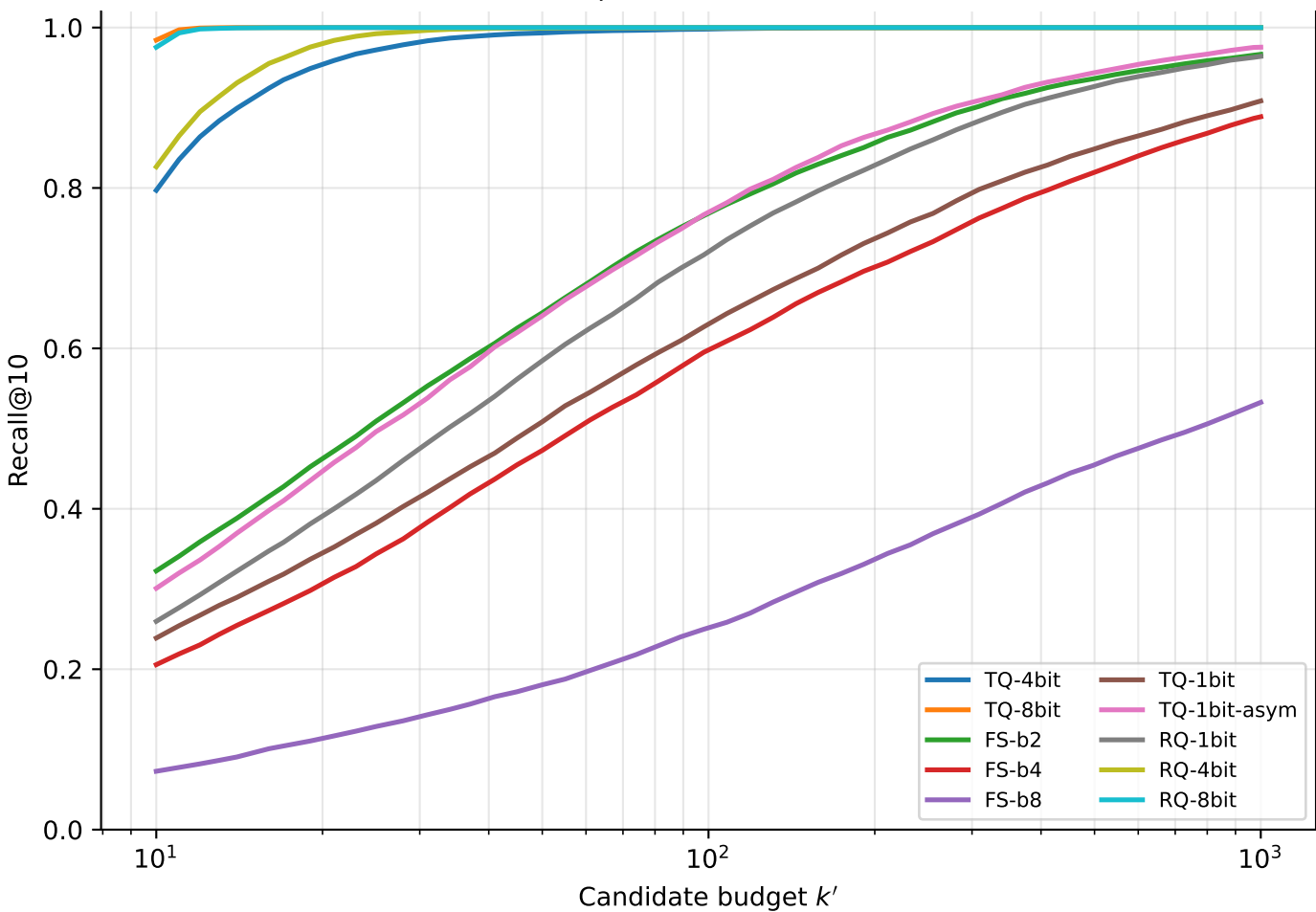
nq: Recall@10 vs k'
