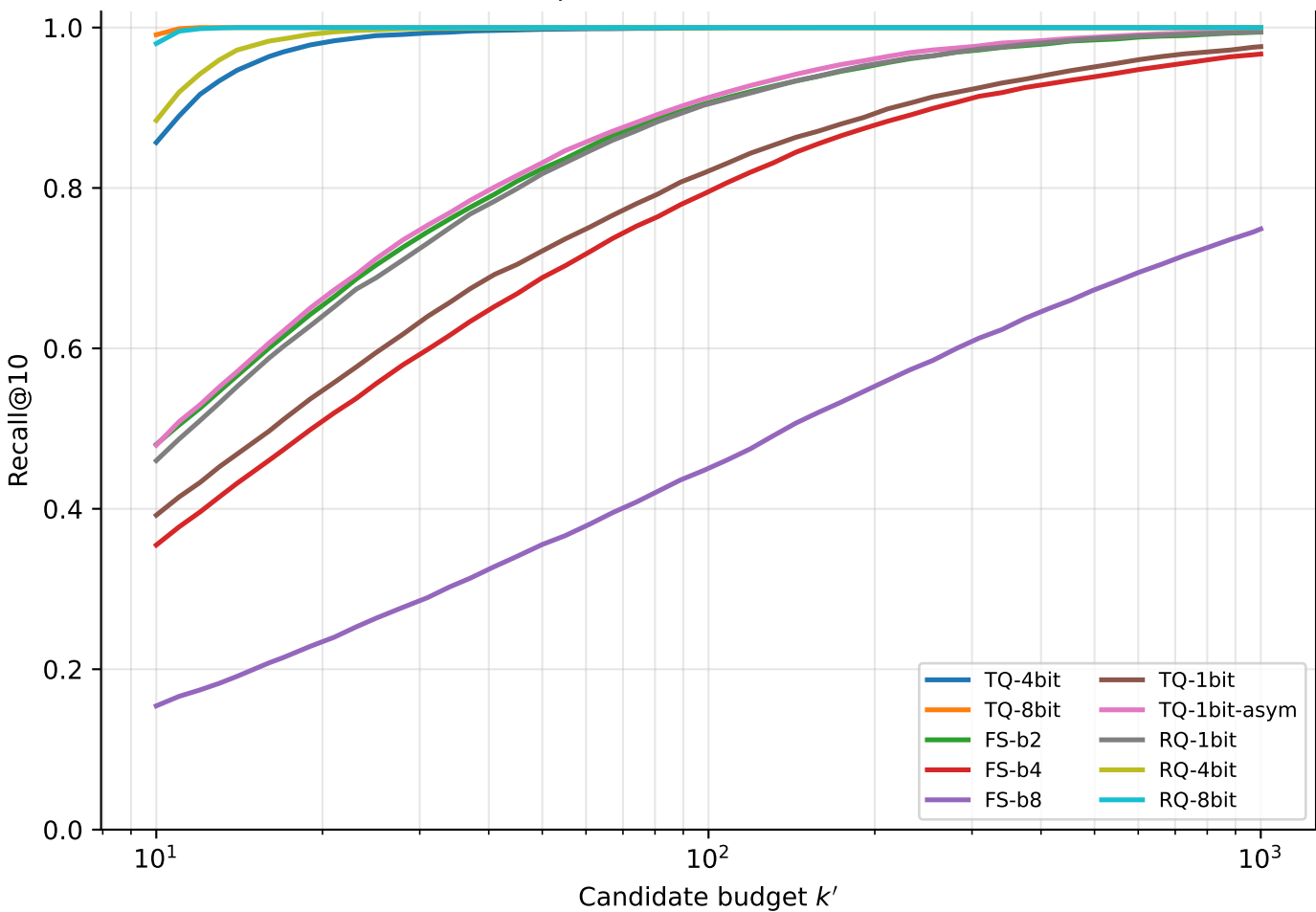
quora: Recall@10 vs k'
