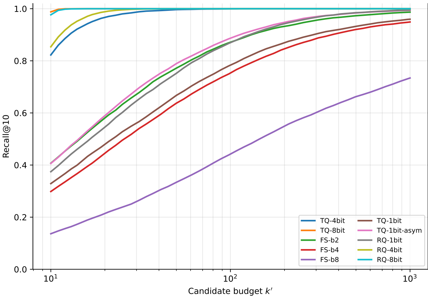
scidocs: Recall@10 vs k'
