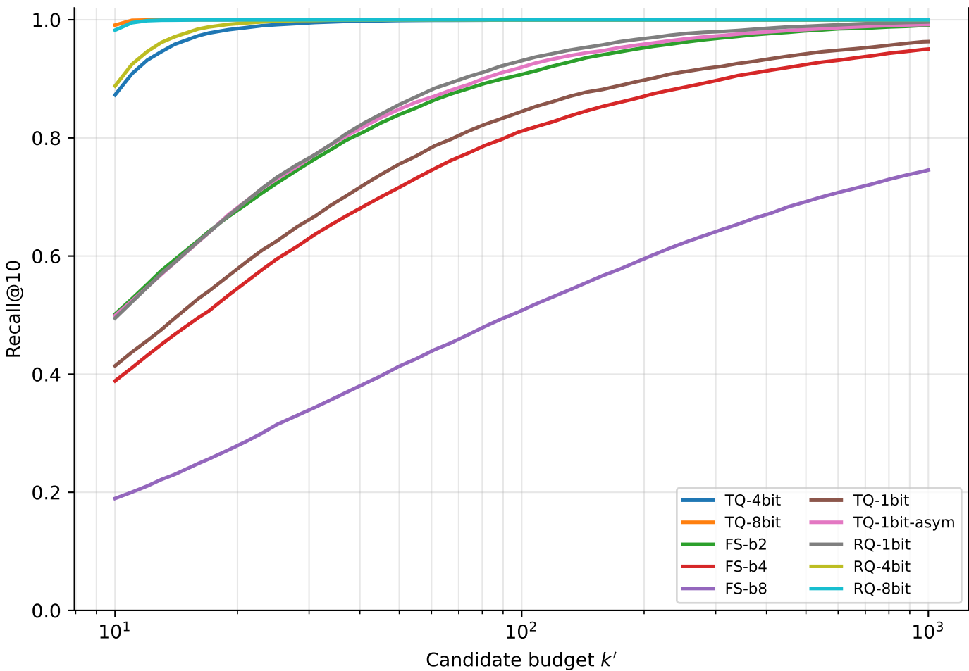
scifact: Recall@10 vs k'
