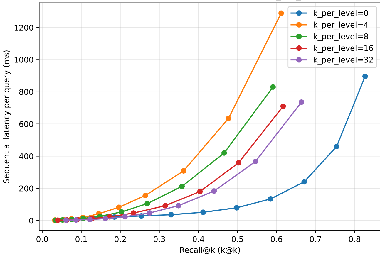
stage1: latency vs recall (grouped by k_per_level)
