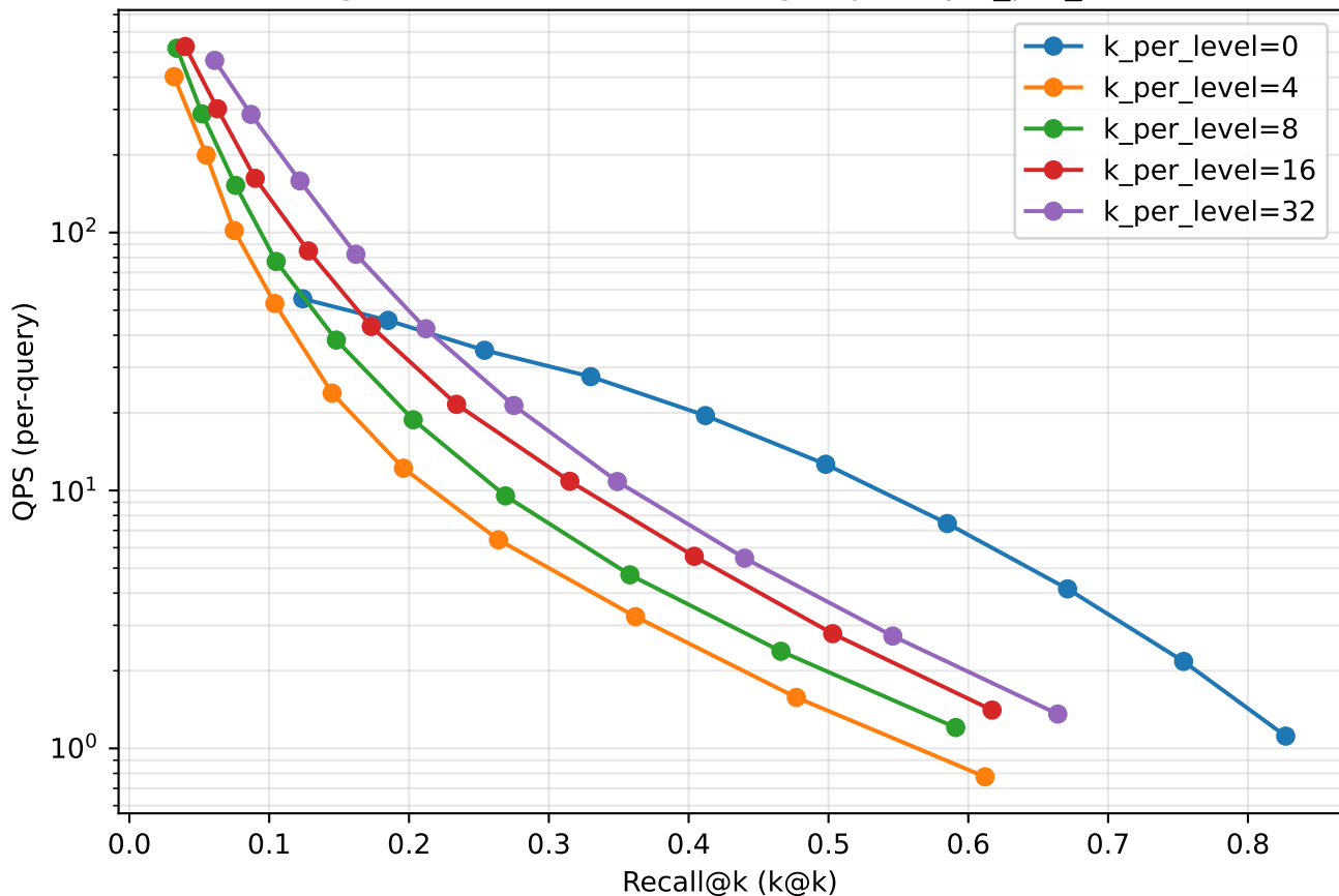
stage1: QPS vs recall Pareto (grouped by k_per_level)
