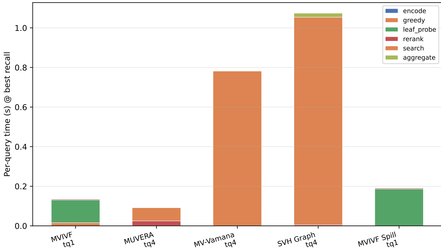
nq: timer breakdown [latency]
