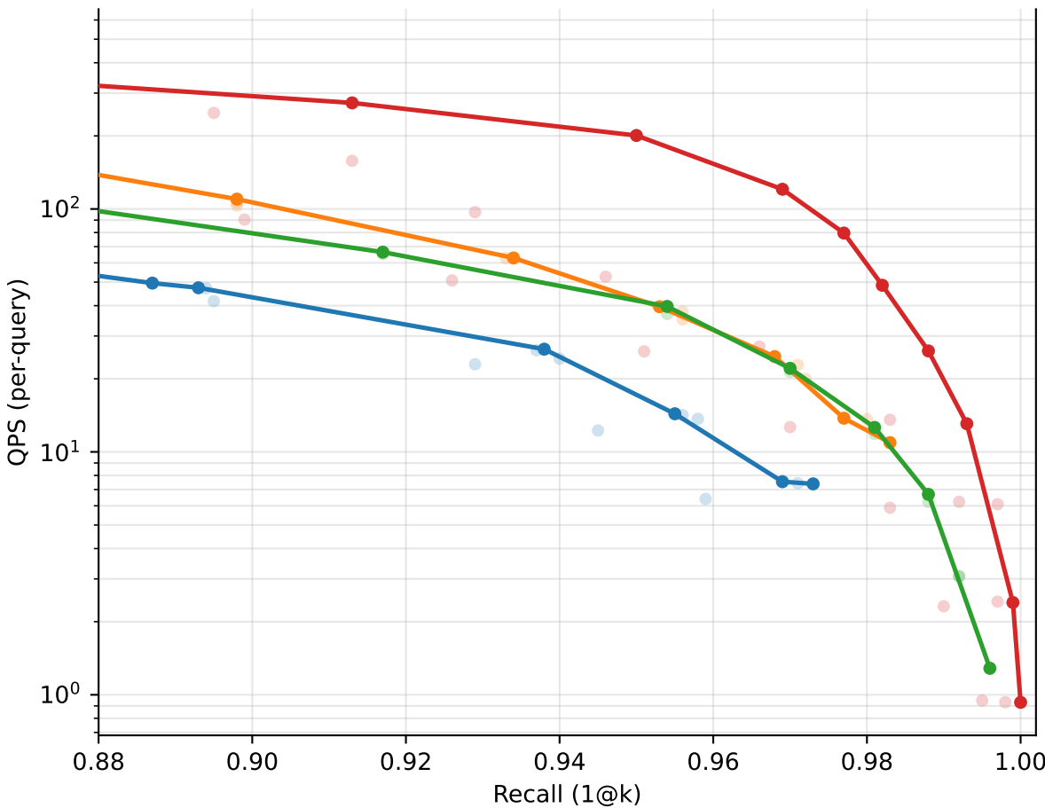
nq: recall vs QPS [latency]
