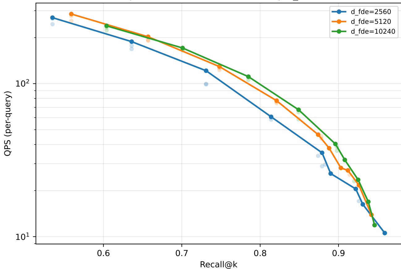
fiqa: MUVERA ablation (Pareto by d_fde)
