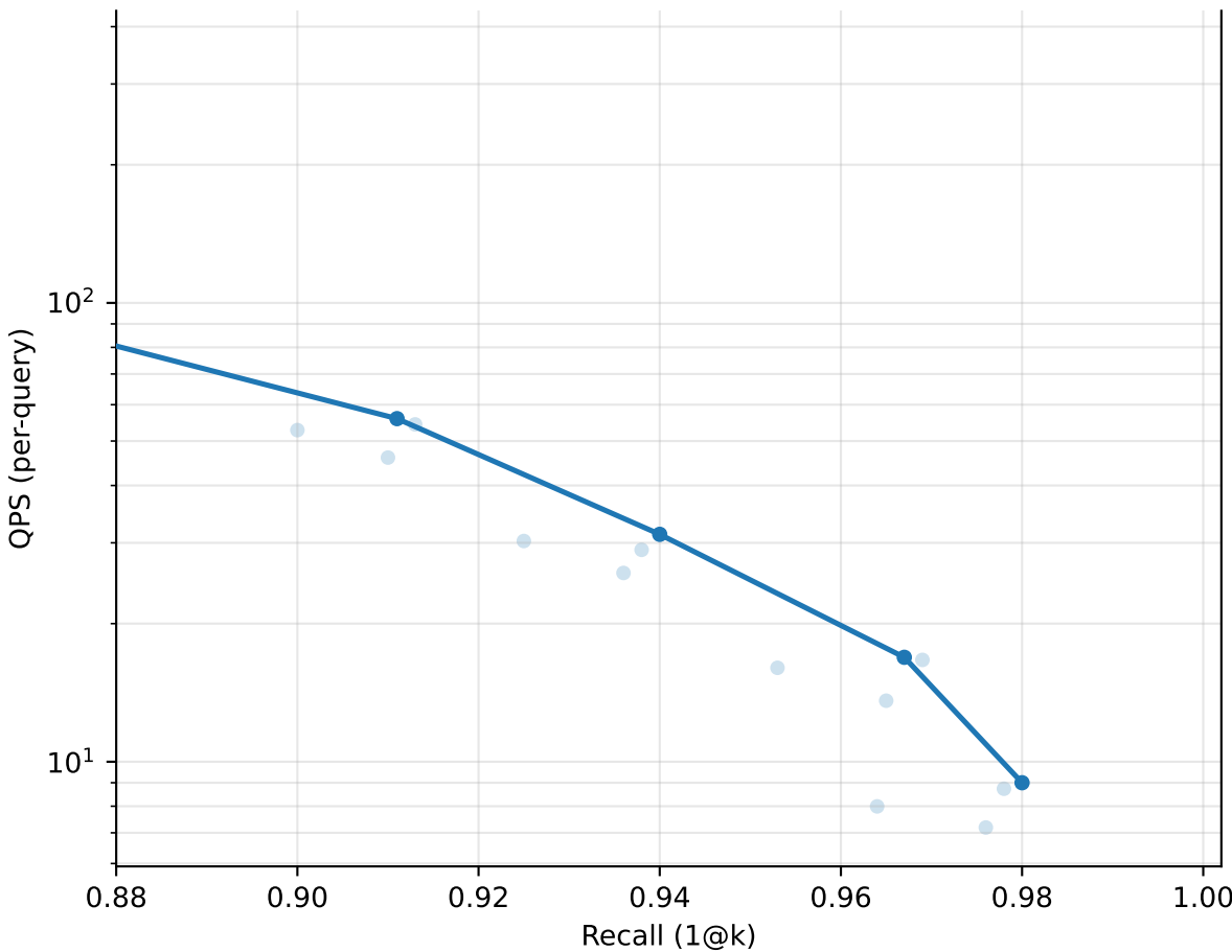
msmarco: recall vs QPS [latency]
