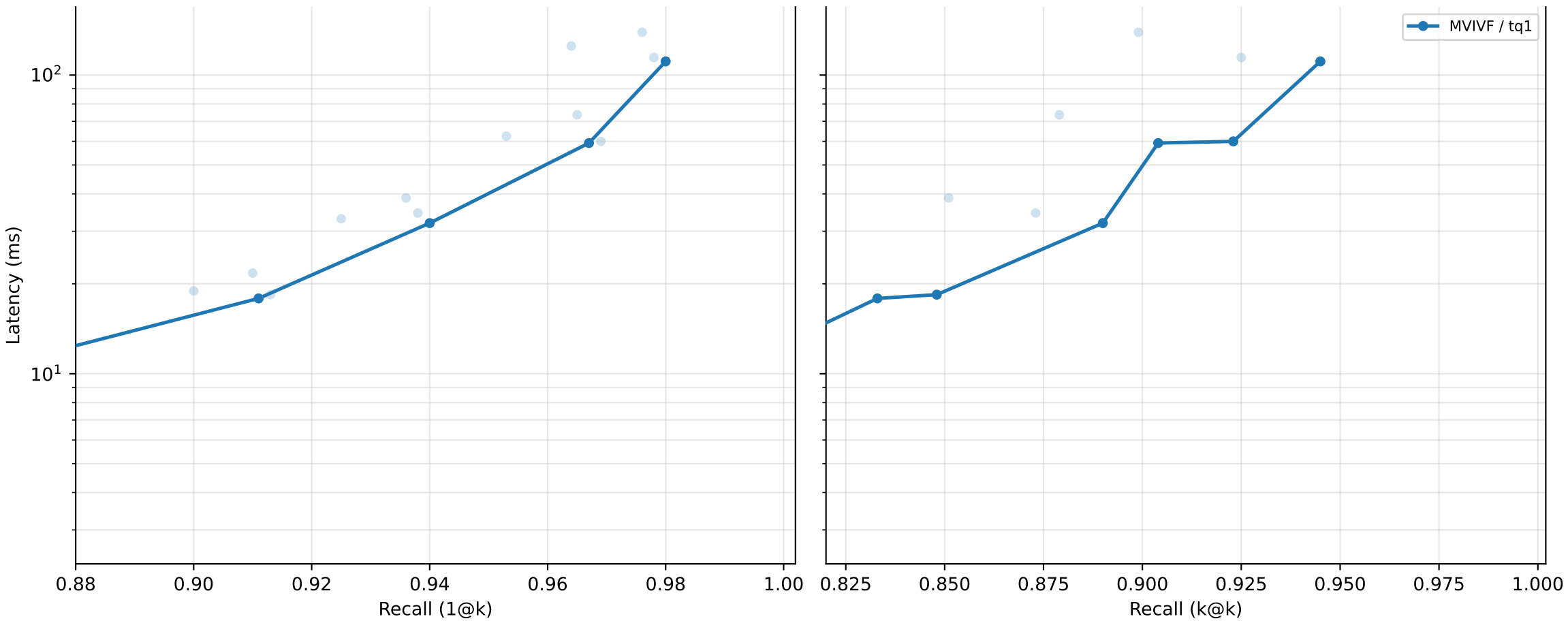
msmarco: recall vs latency (1000 / QPS_seq ms) [latency]
