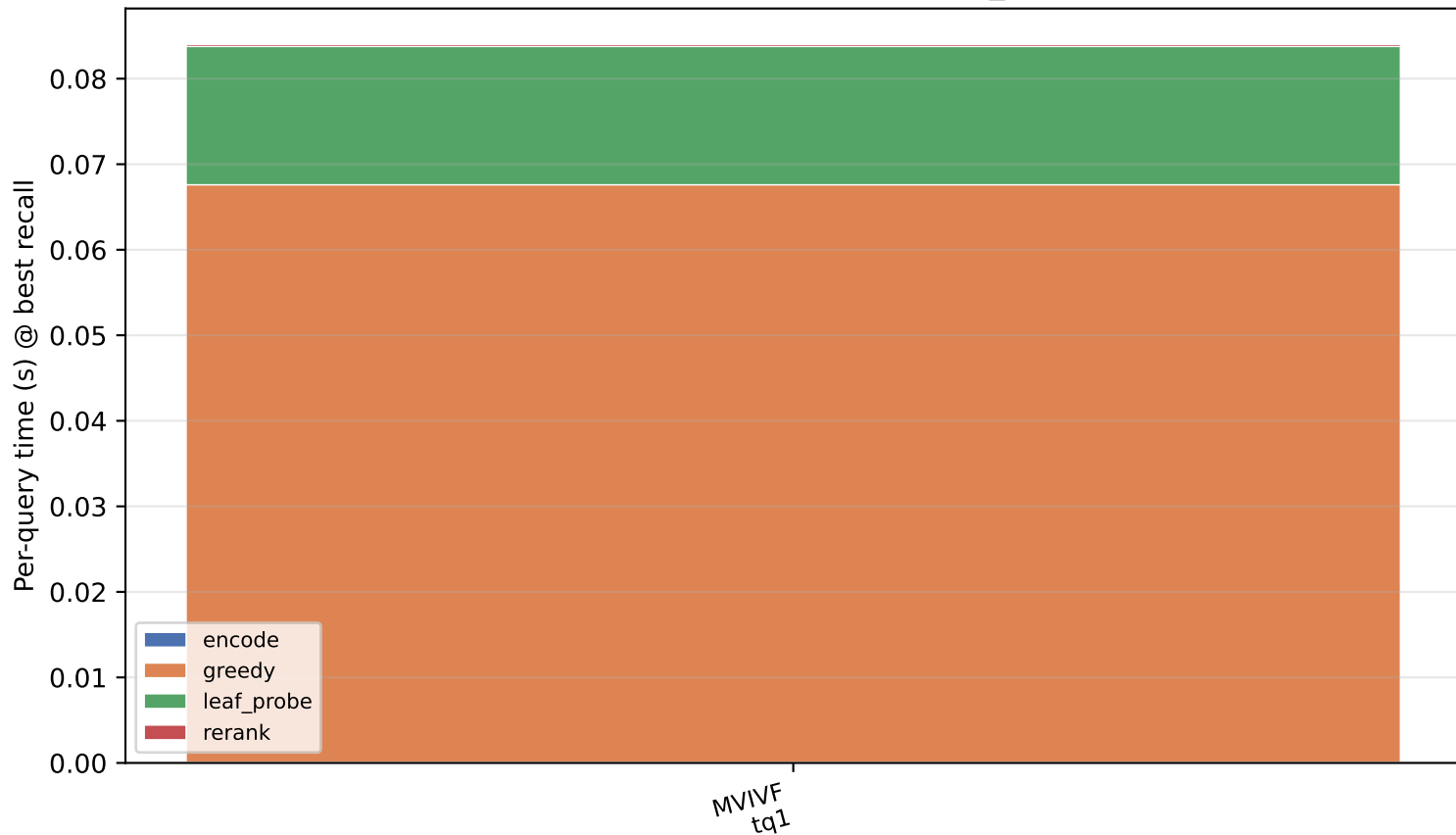
msmarco: timer breakdown [multi_latency]
