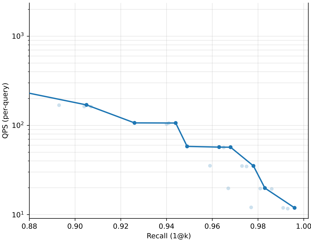
msmarco: recall vs QPS [multi_latency]
