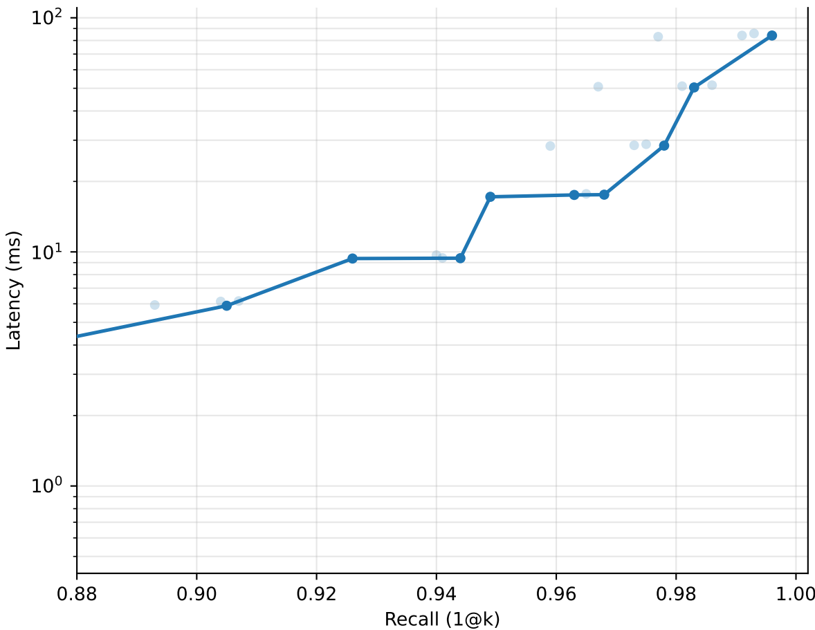
msmarco: recall vs latency (1000 / QPS_seq ms) [multi_latency]
