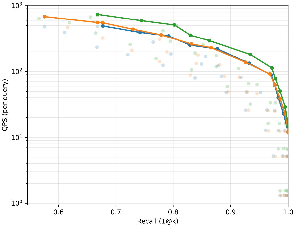
fiqa: SVH Graph ablation Pareto
