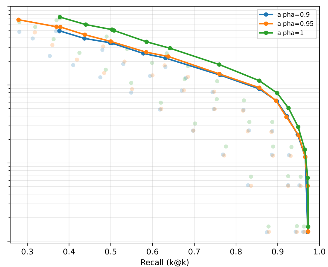
fiqa: SVH Graph ablation Pareto
