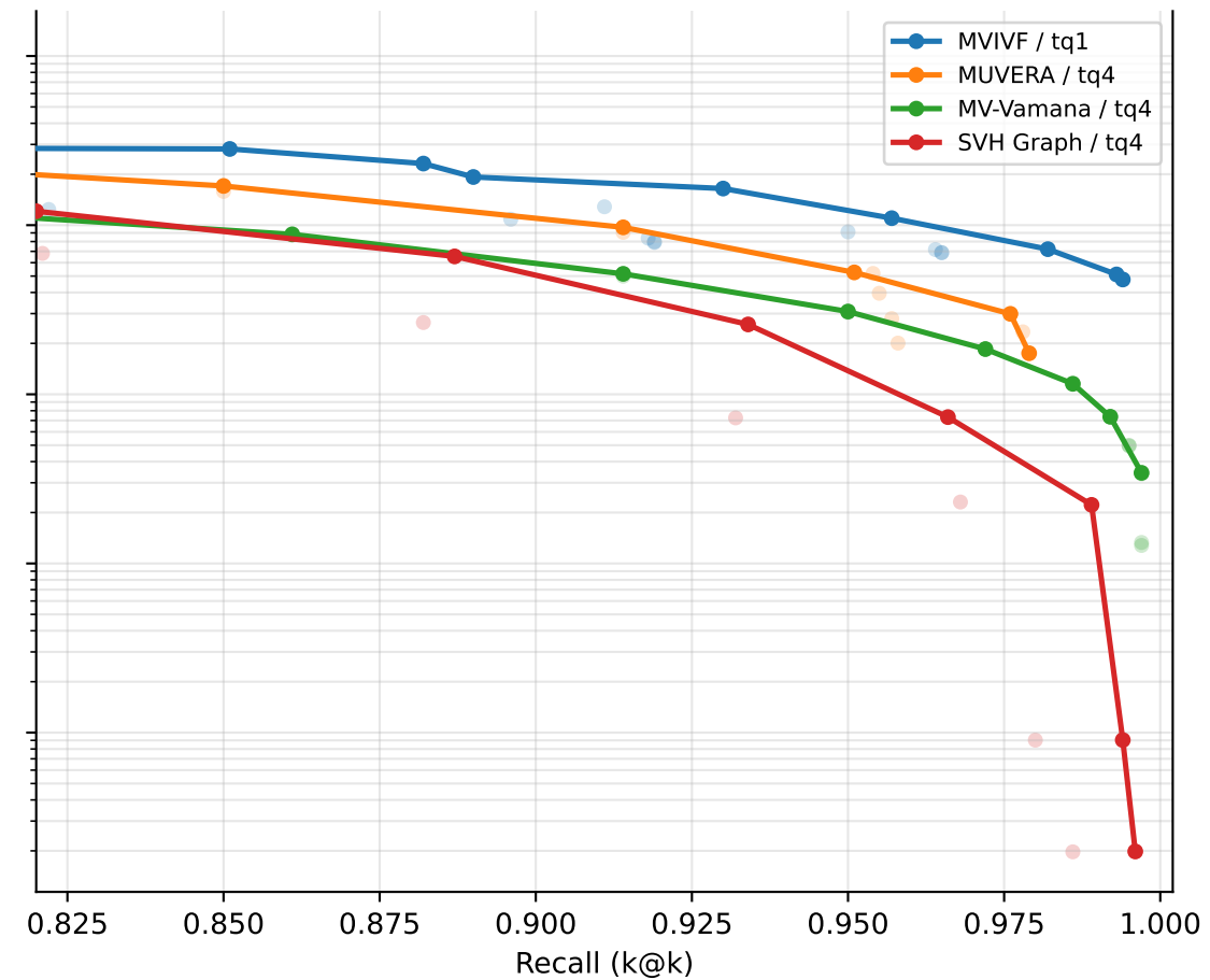
scidocs: recall vs QPS [batch]
