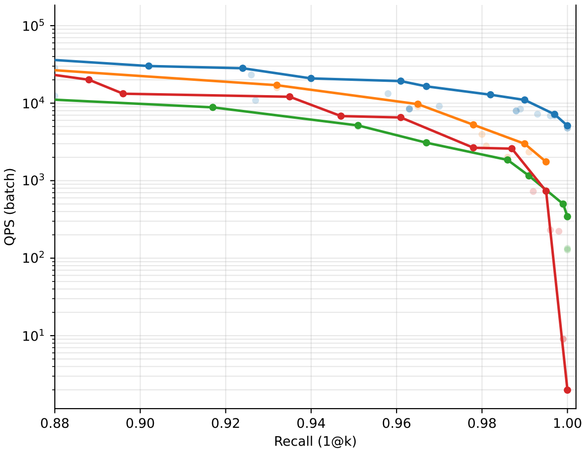
scidocs: recall vs QPS [batch]
