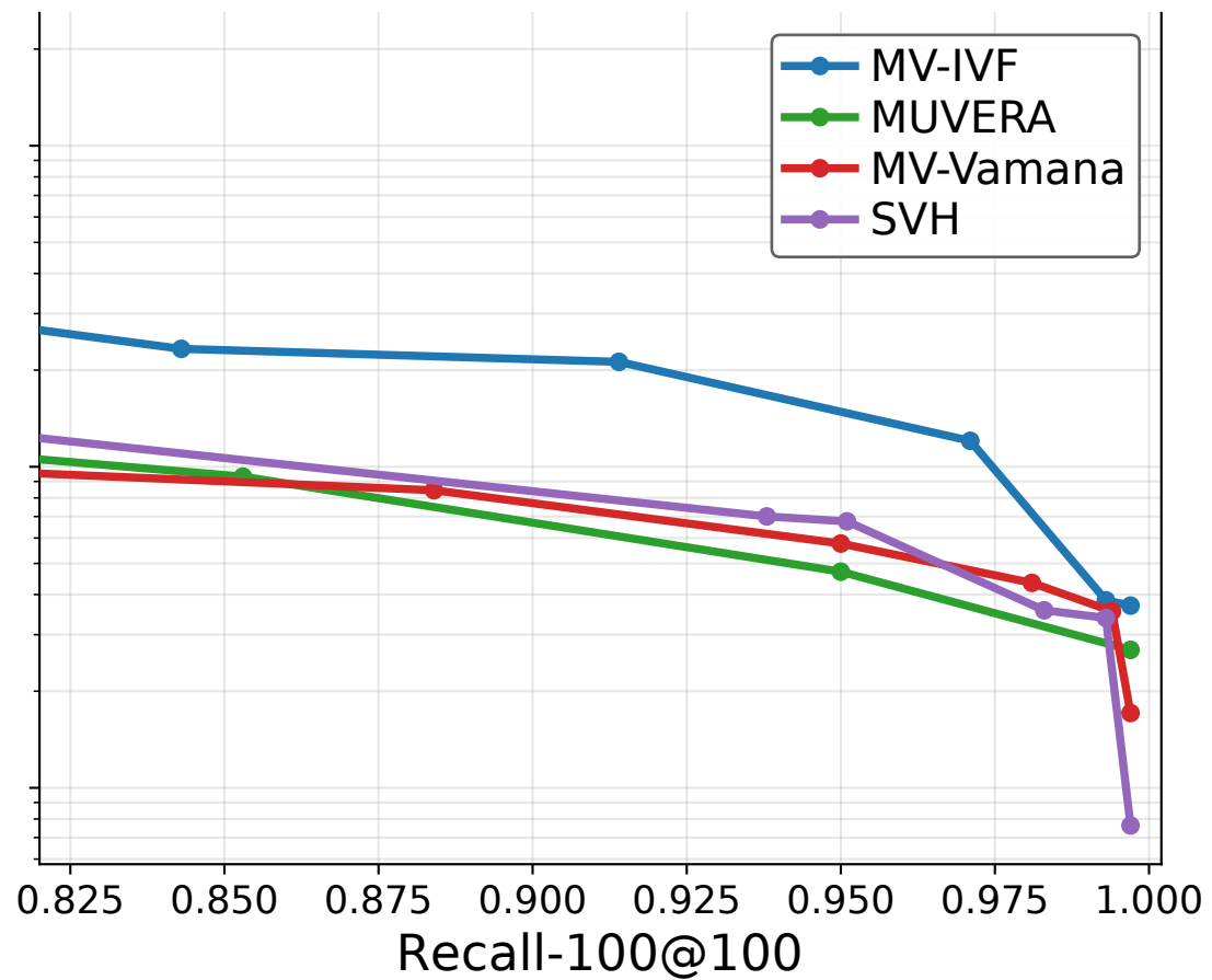
nfcorpus: Recall vs QPS (1 thrd)
