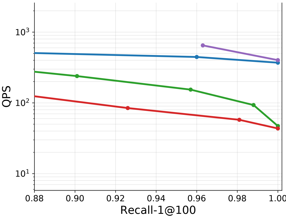
nfcorpus: Recall vs QPS (1 thrd)
