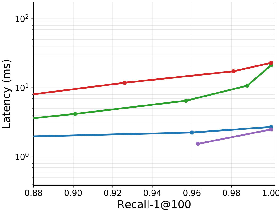
nfcorpus: Recall vs Latency (1 thrd)
