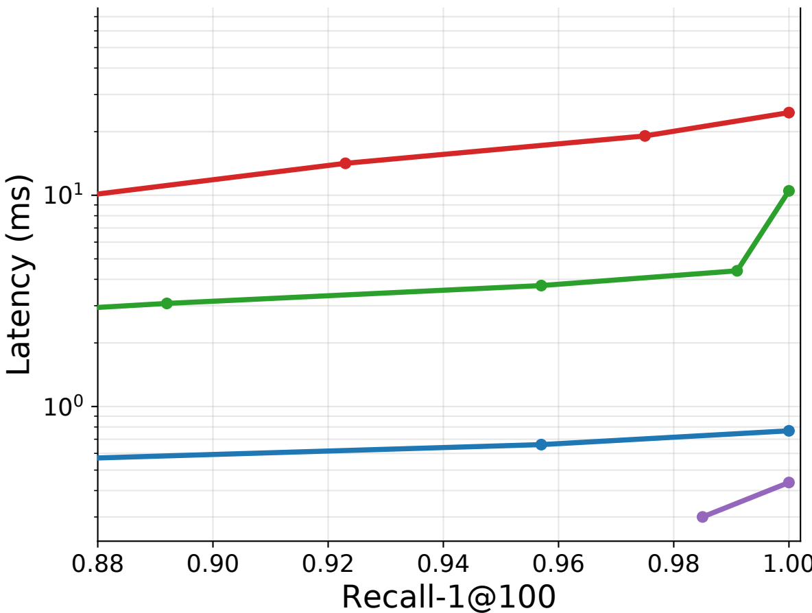
nfcorpus: Recall vs Latency (all thrds)
