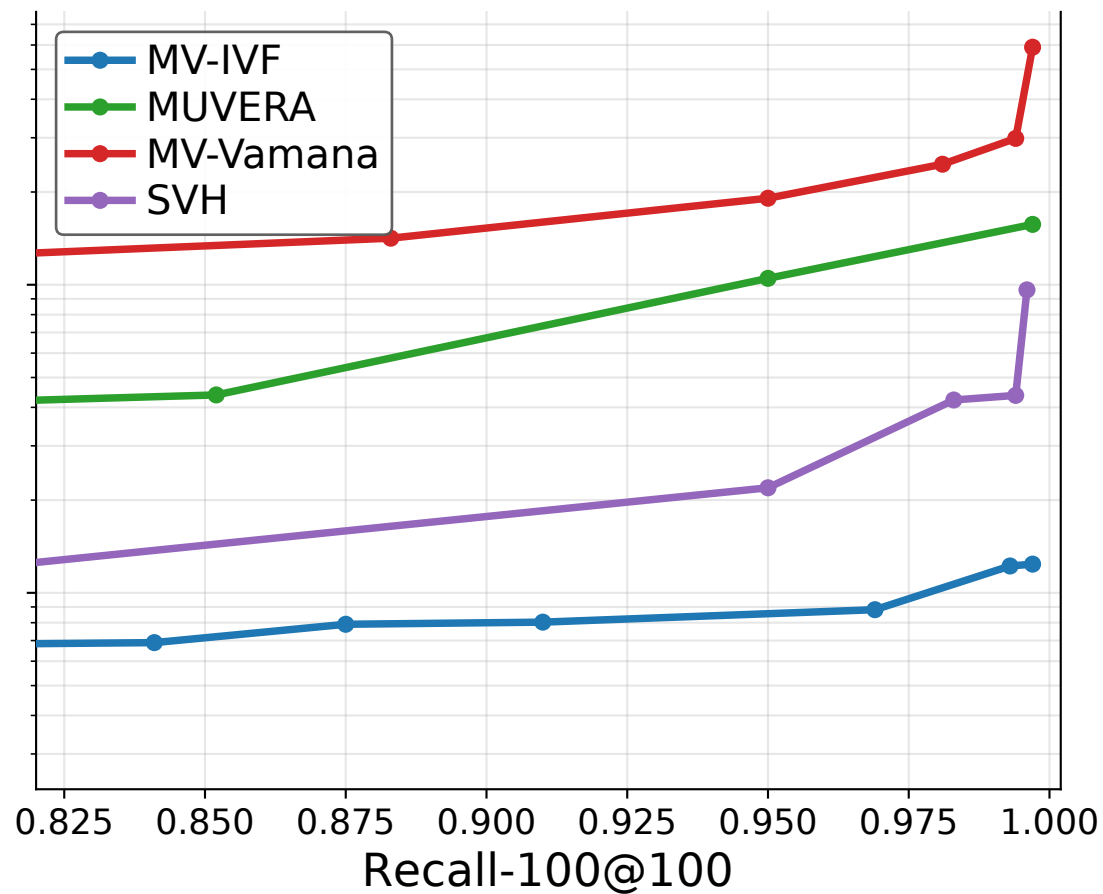
nfcorpus: Recall vs Latency (all thrds)
