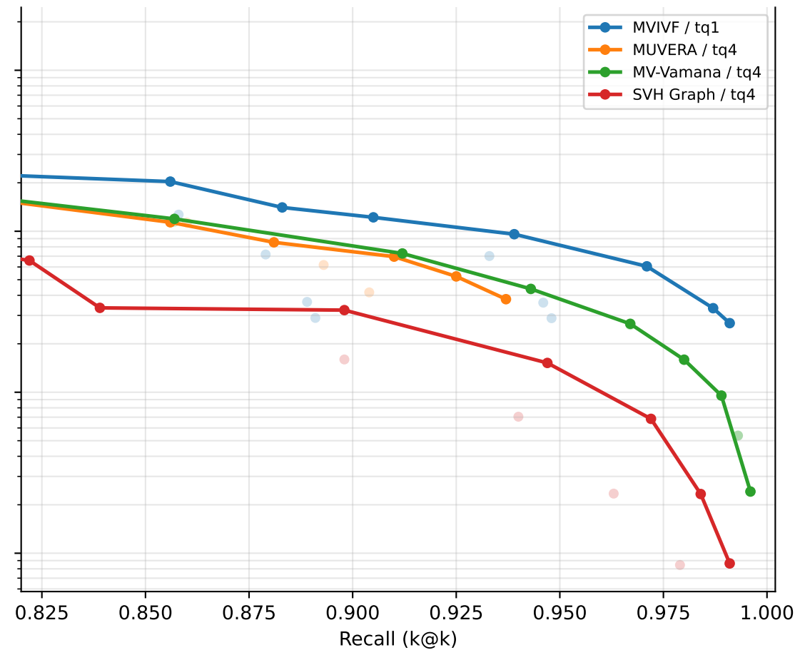
fiqa: recall vs QPS [latency]
