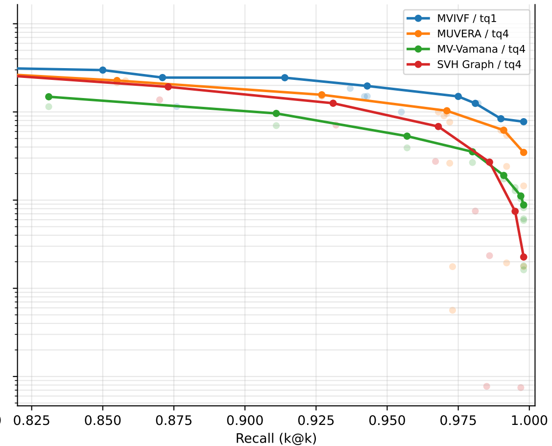
scifact: recall vs QPS [batch]
