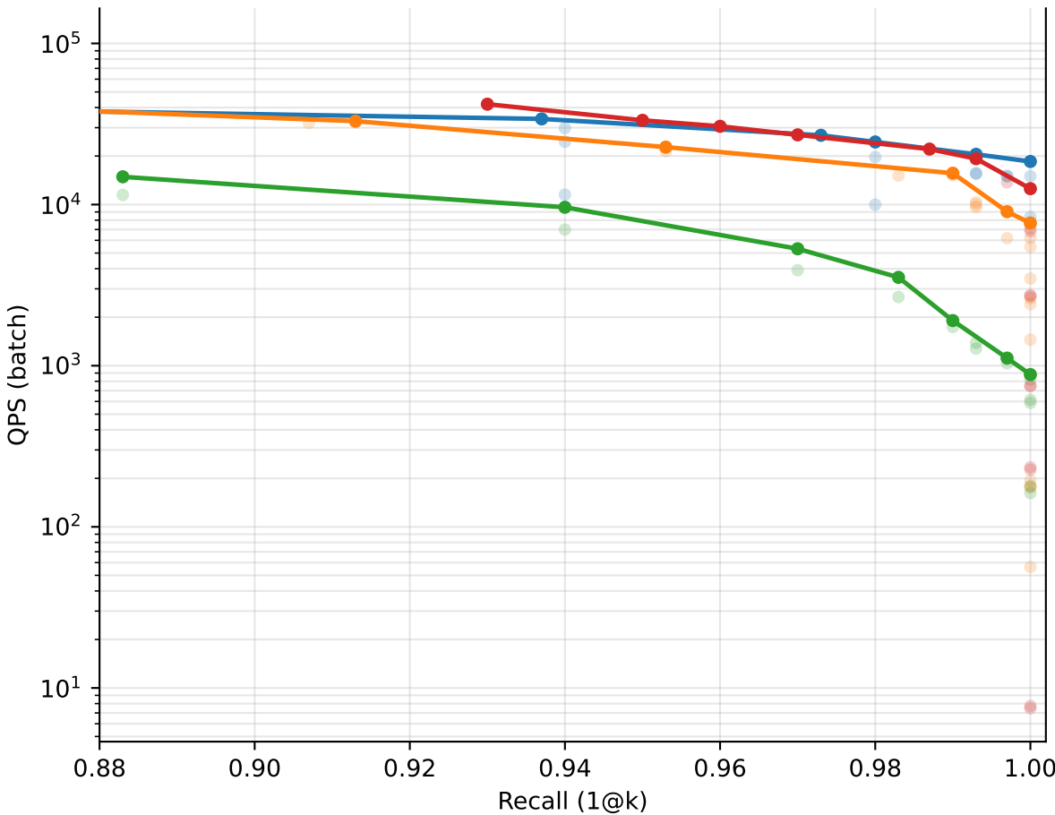
scifact: recall vs QPS [batch]
