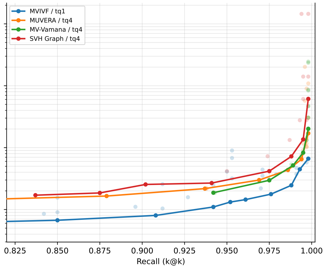
arguana: recall vs latency (1000 / QPS_seq ms) [latency]
