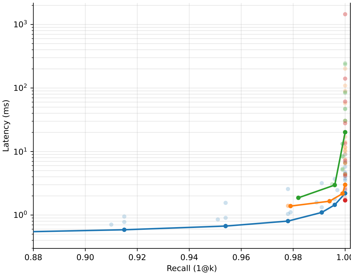
arguana: recall vs latency (1000 / QPS_seq ms) [latency]
