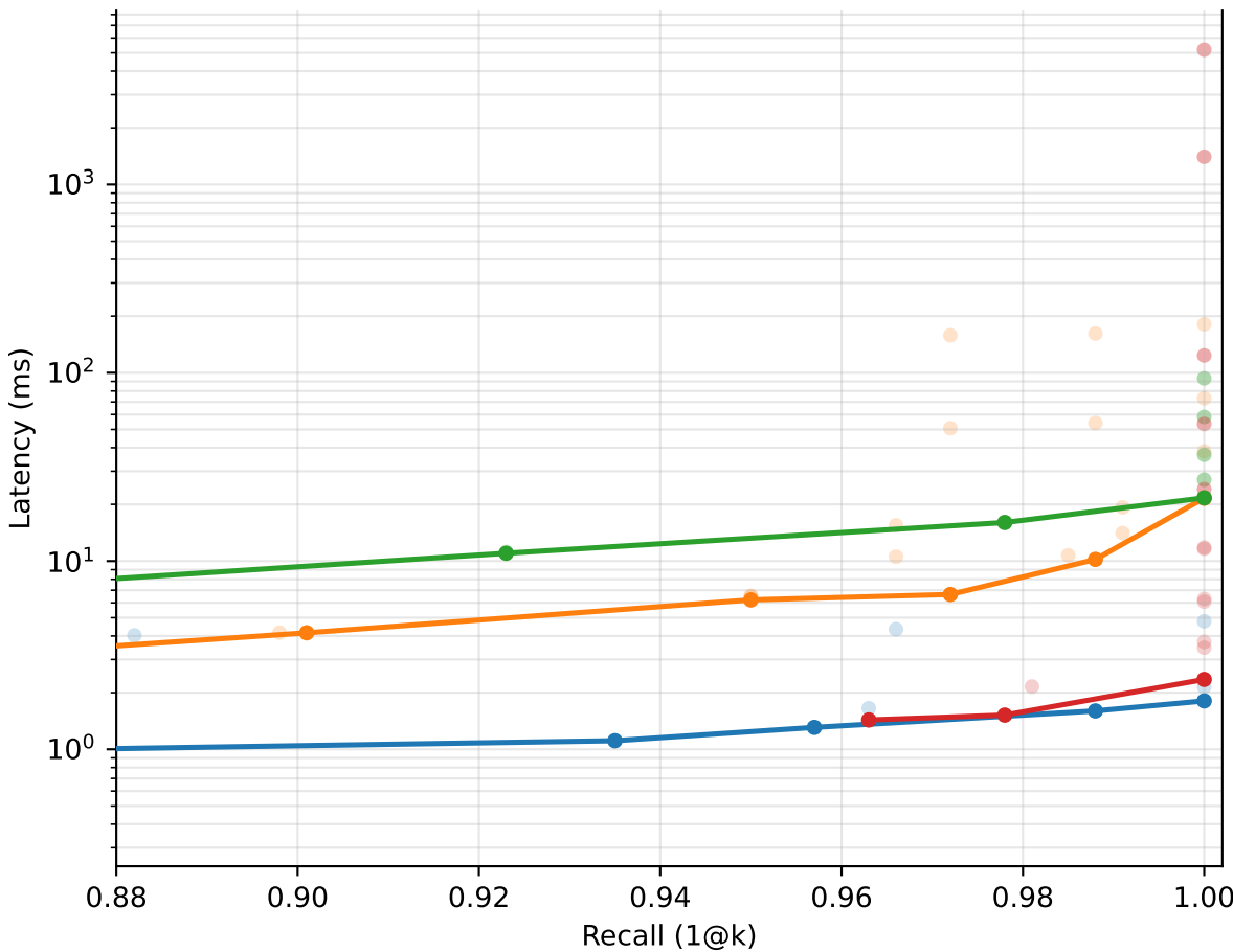
nfcorpus: recall vs latency (1000 / QPS_seq ms) [latency]
