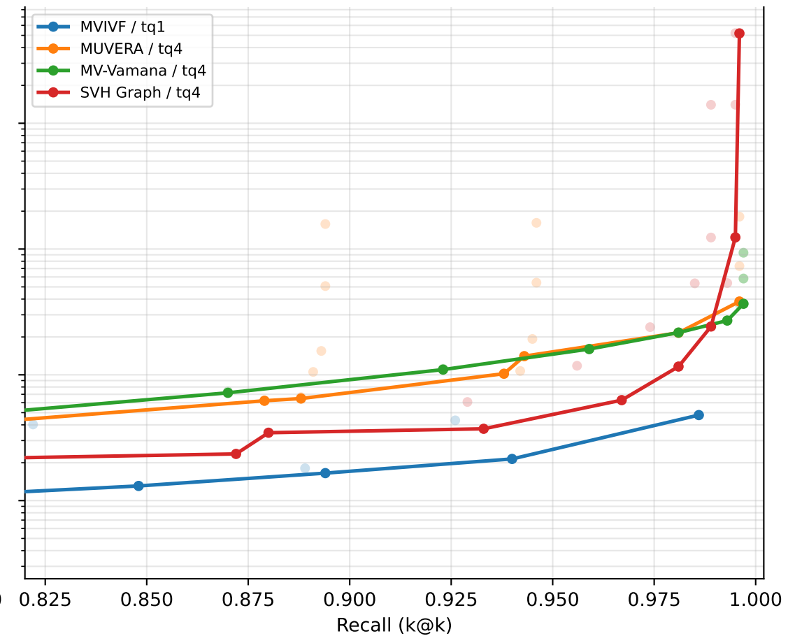
nfcorpus: recall vs latency (1000 / QPS_seq ms) [latency]
