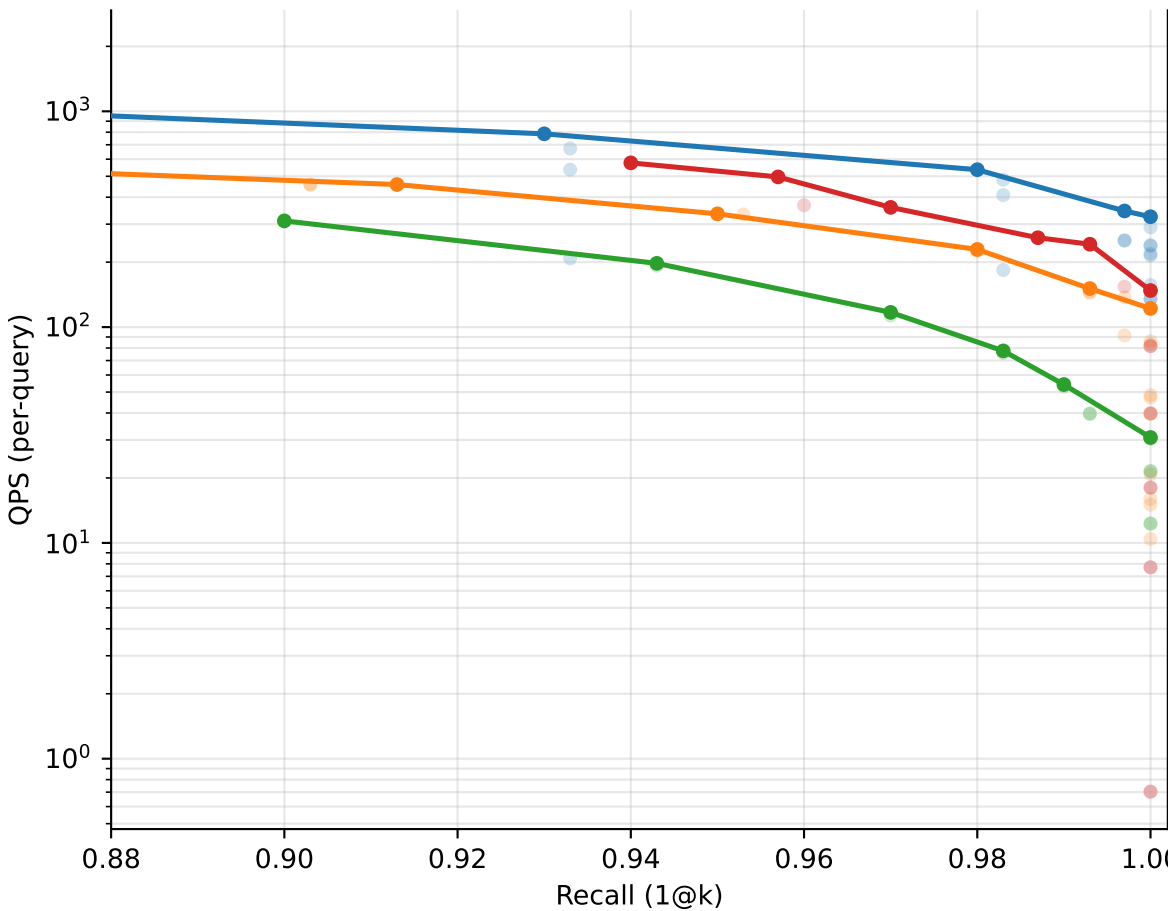
scifact: recall vs QPS [latency]
