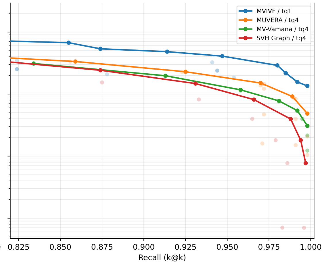
scifact: recall vs QPS [latency]
