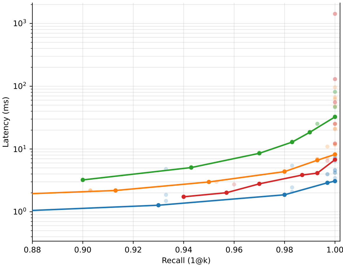
scifact: recall vs latency (1000 / QPS_seq ms) [latency]
