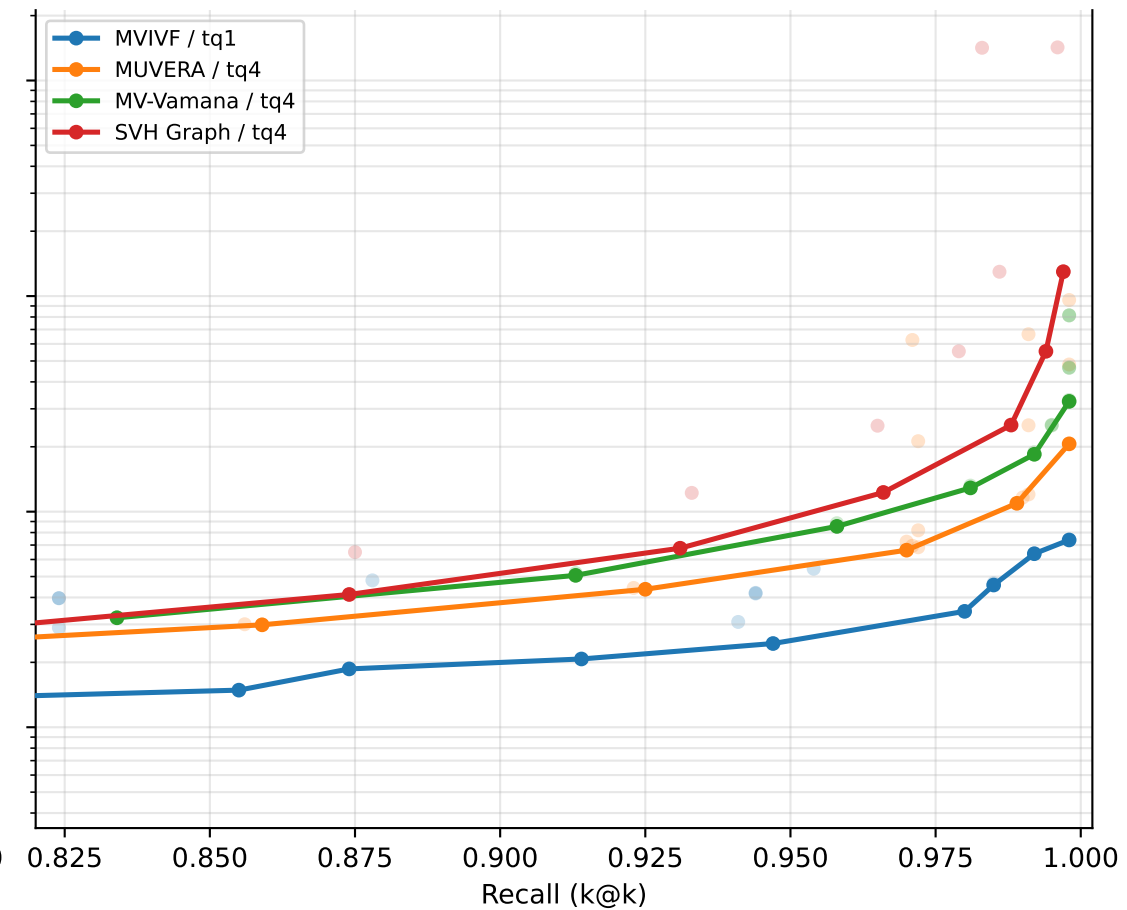
scifact: recall vs latency (1000 / QPS_seq ms) [latency]
