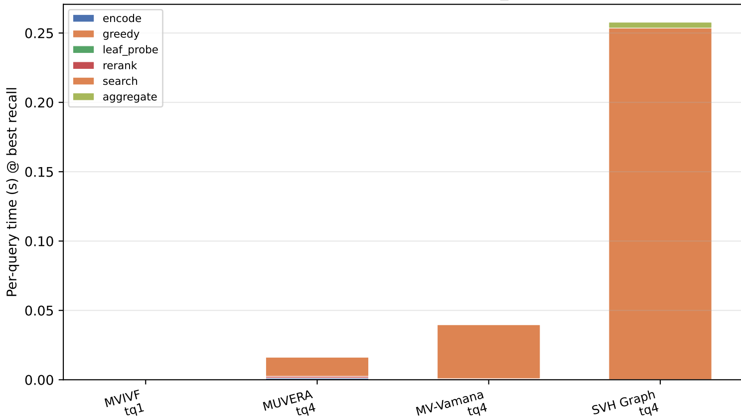
nfcorpus: timer breakdown [multi_latency]
