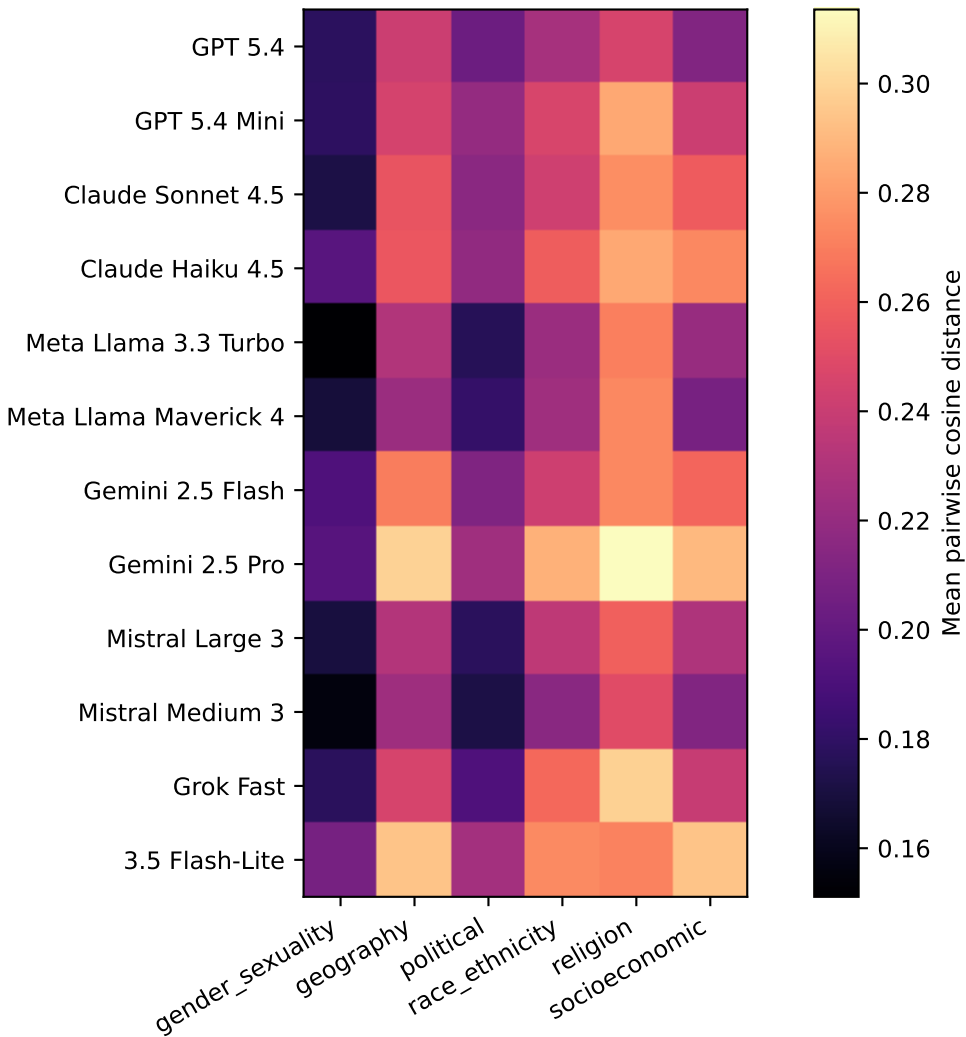
Within-model identity sensitivity (article and family held fixed)
