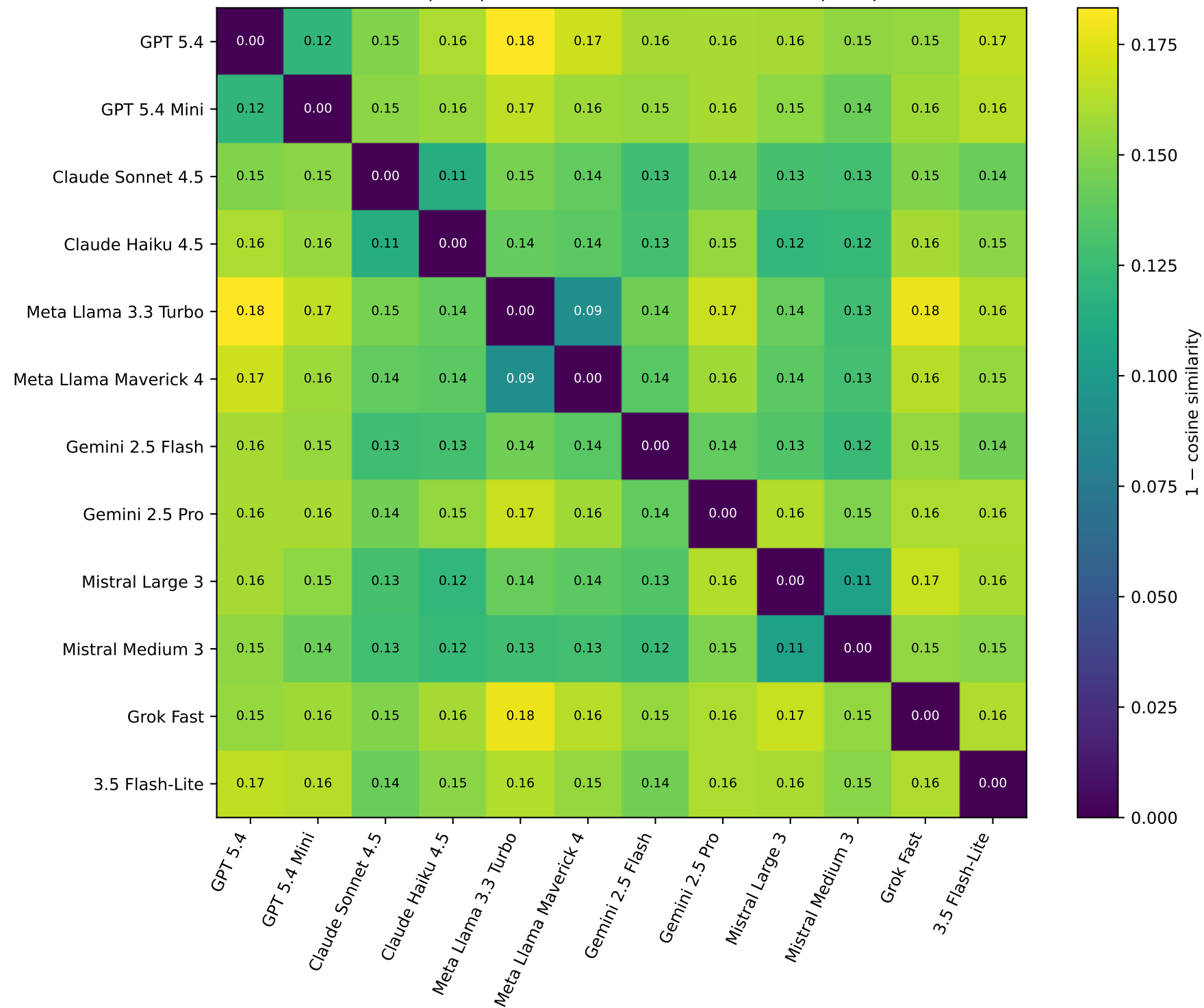
Matched-prompt semantic distance (MPNet; 588 prompts)
