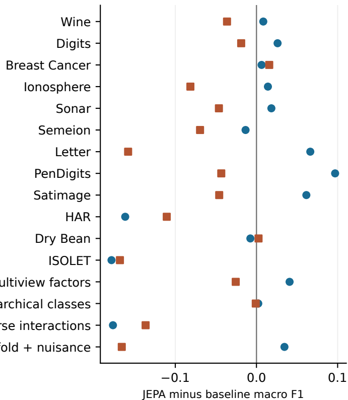
Classification (16 datasets)
