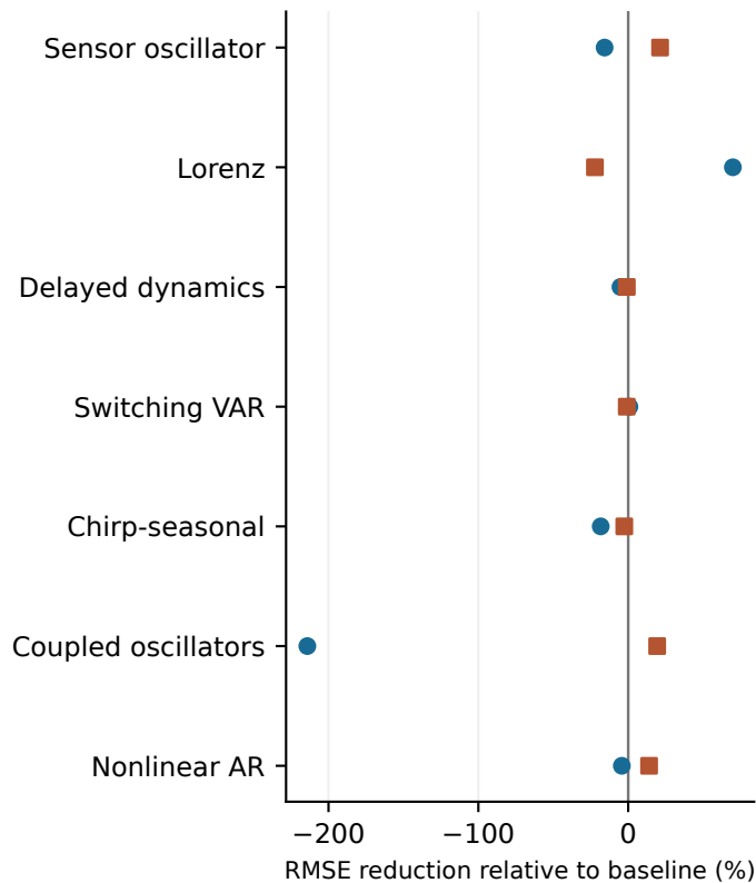
Forecasting (7 datasets)
