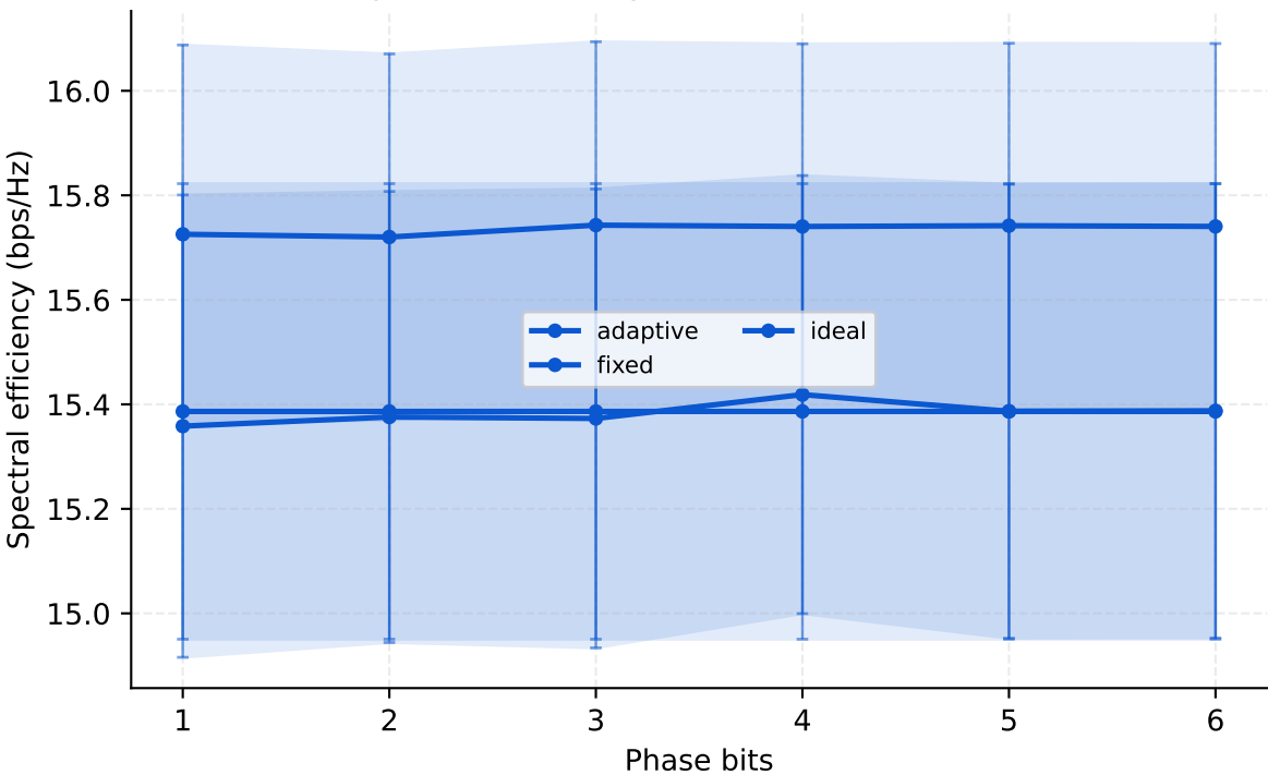
Spectral Efficiency versus Phase Resolution
